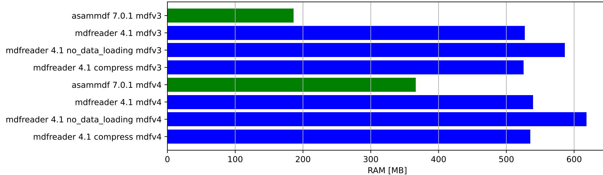
Save test file - ram usage
