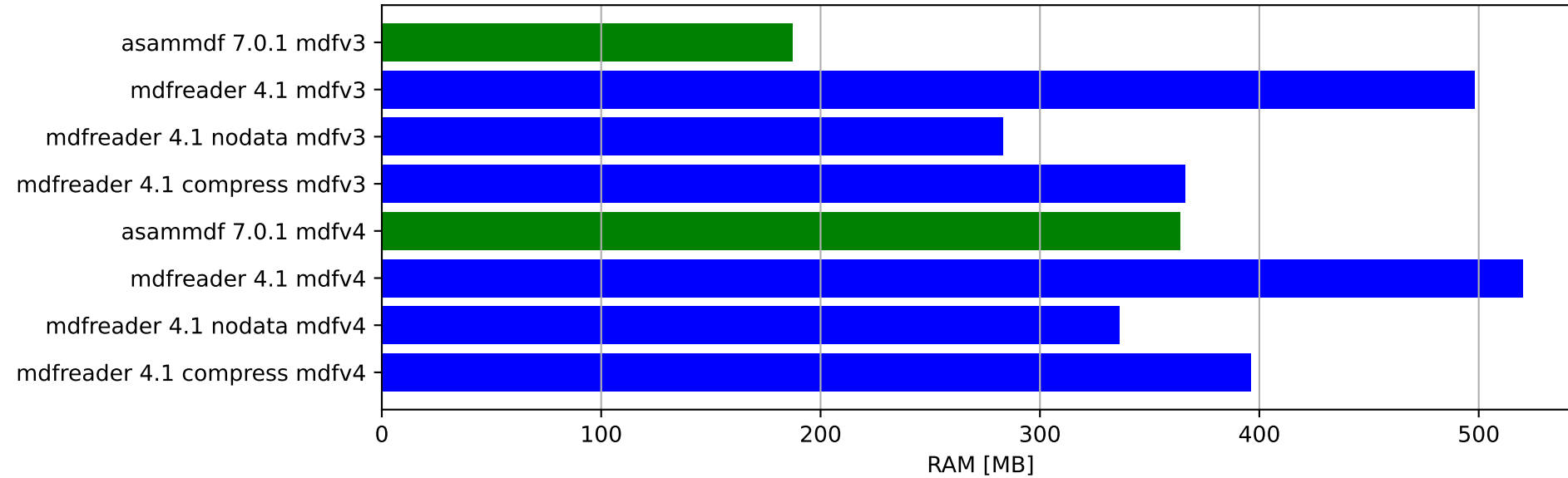
Get all channels (36424 calls) - ram usage
