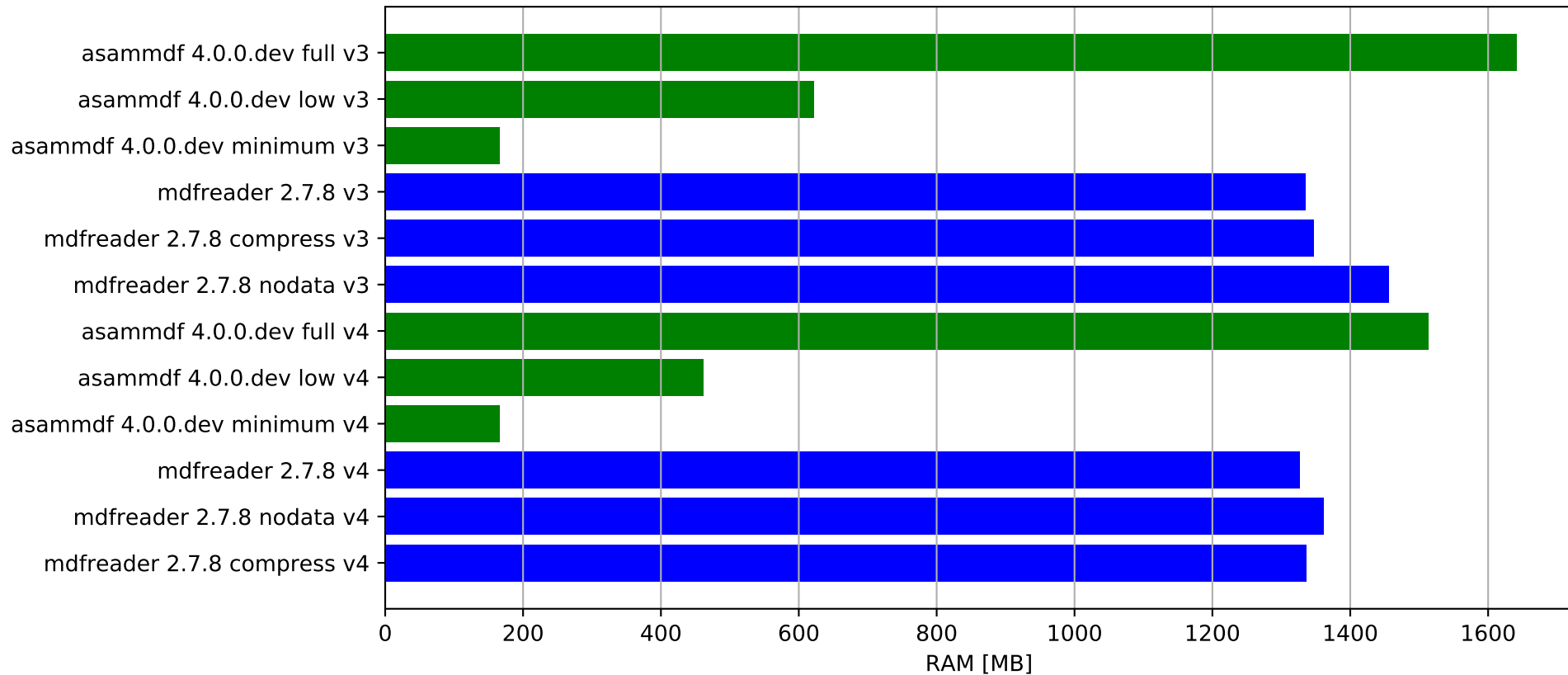
Merge test file - ram usage
