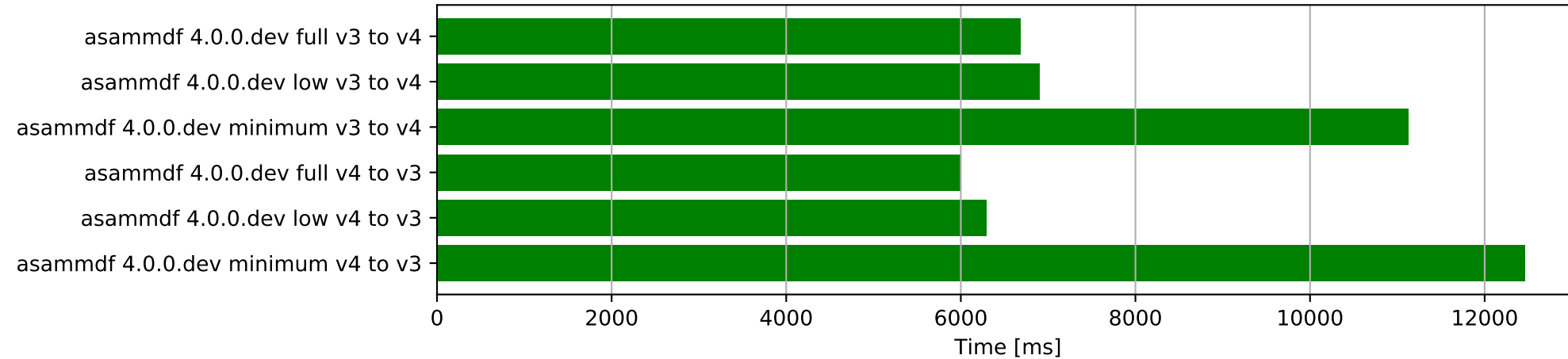
Convert test file - time
