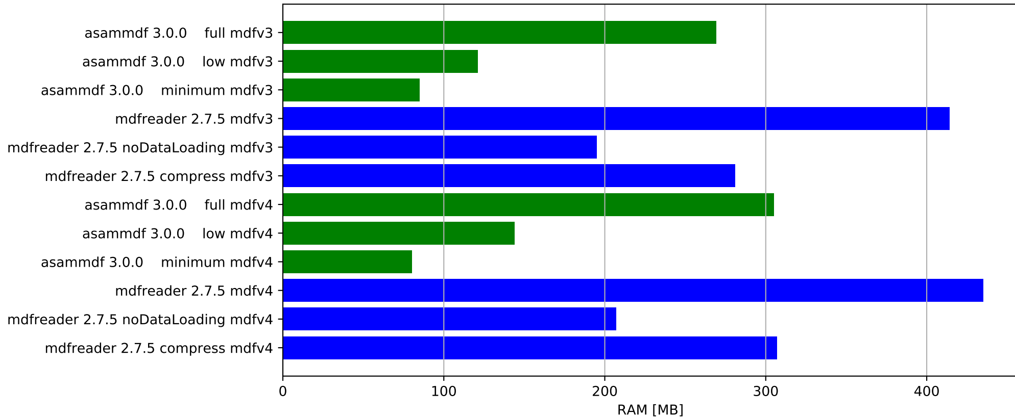
Get all channels (36424 calls) - ram usage
