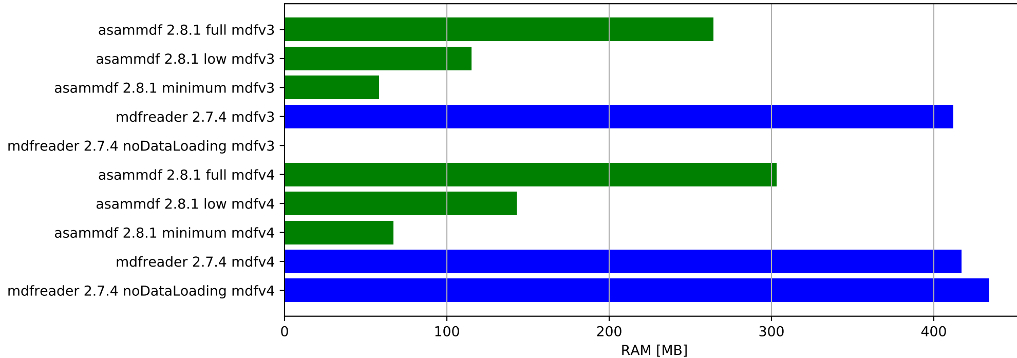
Save test file - ram usage
