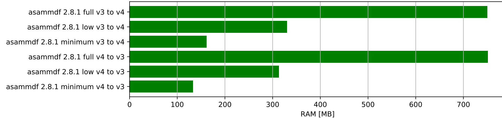
Convert test file - ram usage
