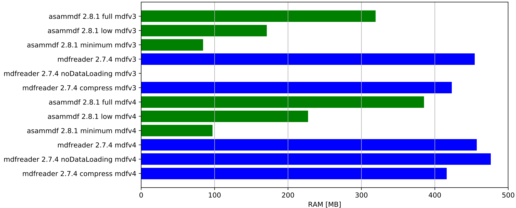
Save test file - ram usage
