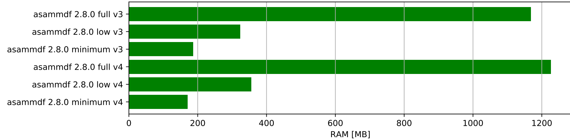
Merge test file - ram usage
