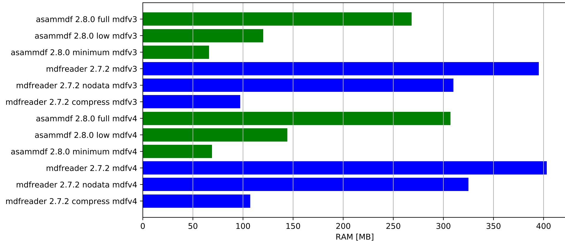
Get all channels (36424 calls) - ram usage
