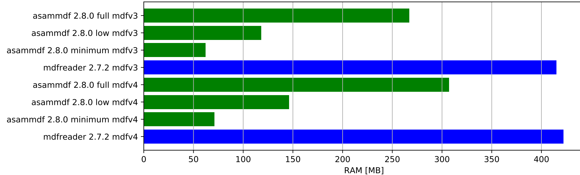
Save test file - ram usage
