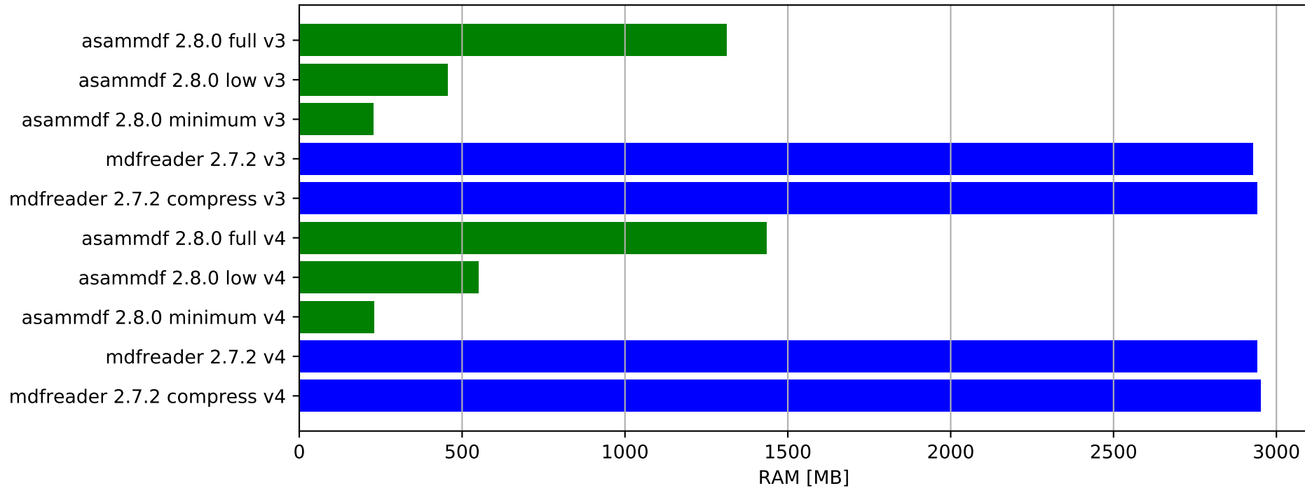
Merge test file - ram usage
