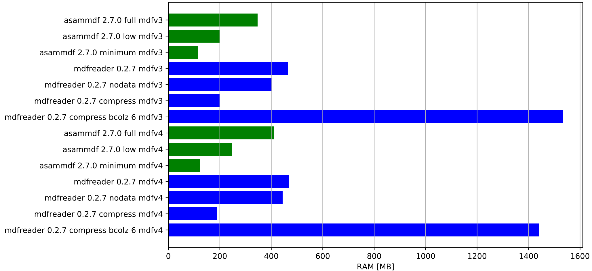
Get all channels (36424 calls) - ram usage
