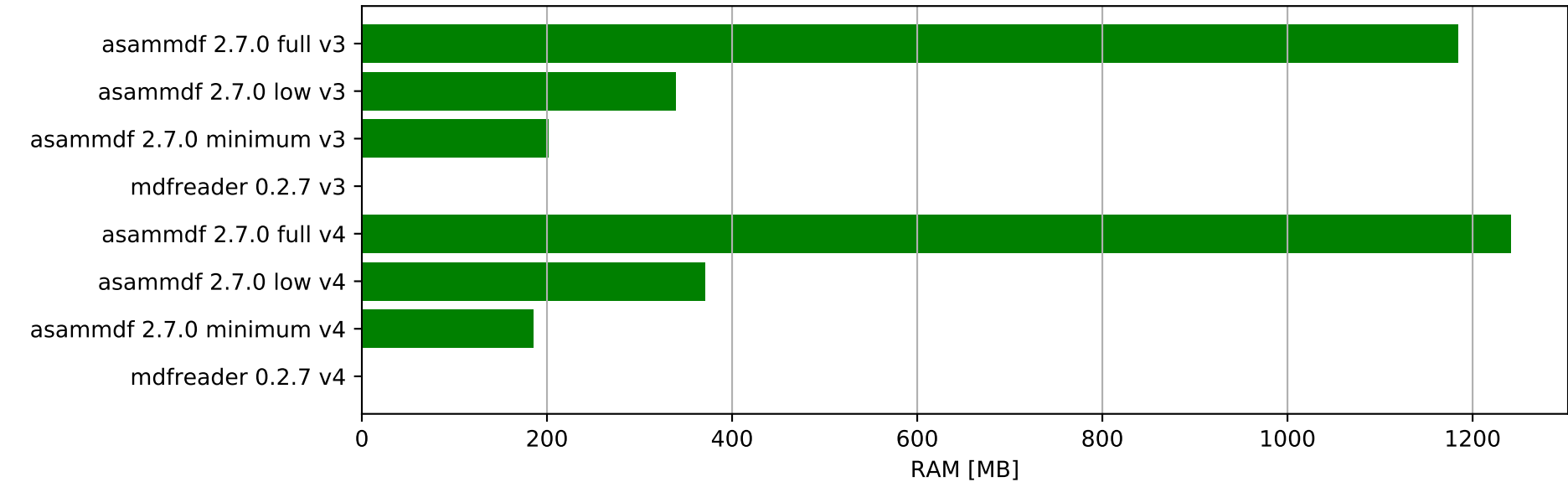
Merge test file - ram usage
