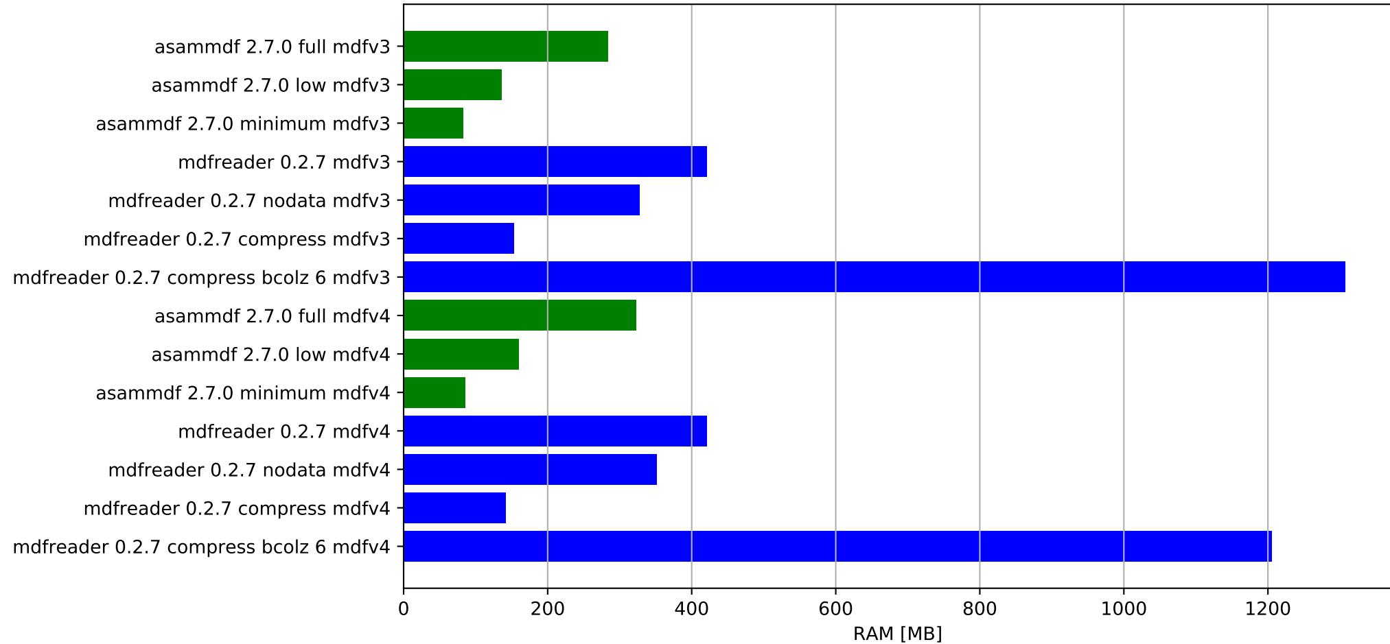
Get all channels (36424 calls) - ram usage
