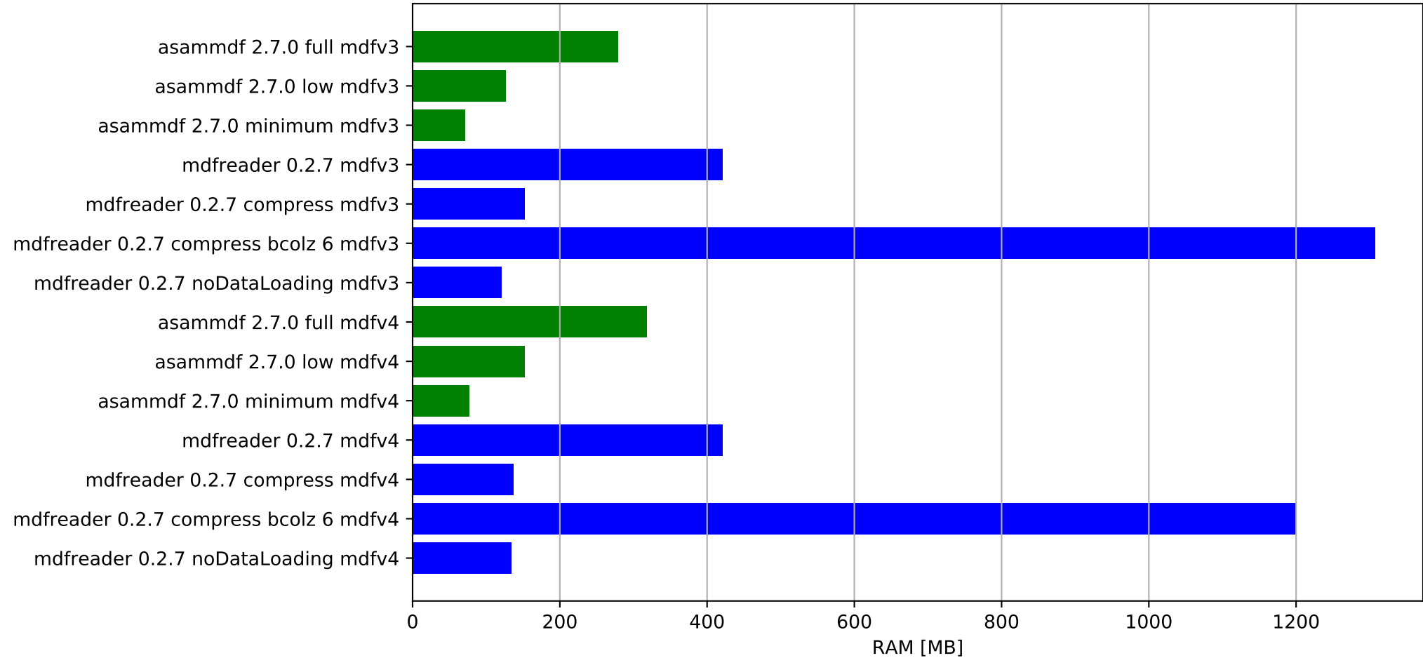
Open test file - ram usage
