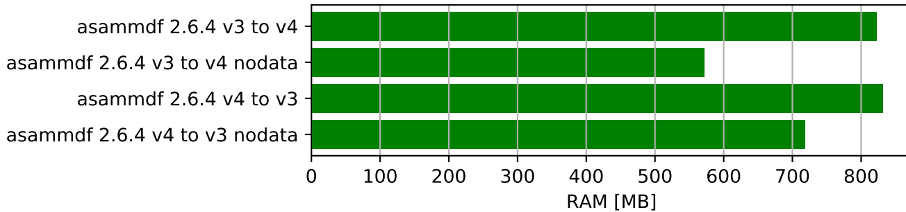
Convert test file - ram usage
