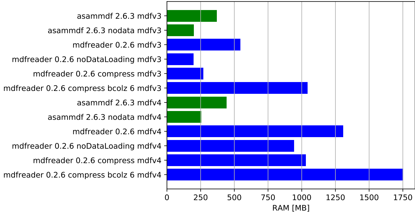
Get all channels (36424 calls) - ram usage
