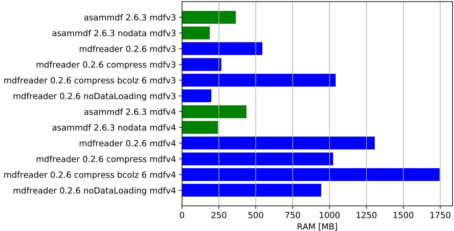
Open test file - ram usage
