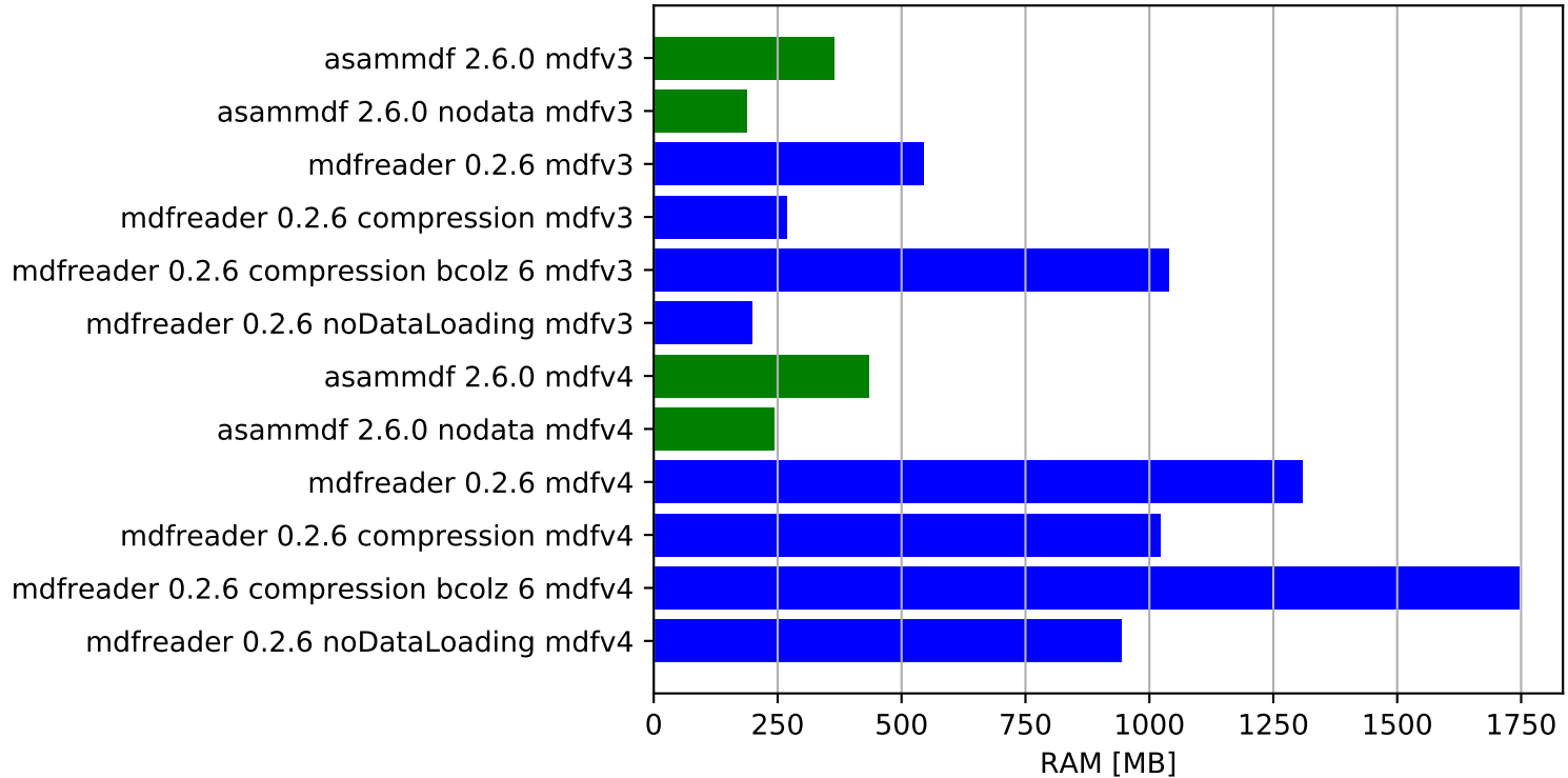
Open test file - ram usage
