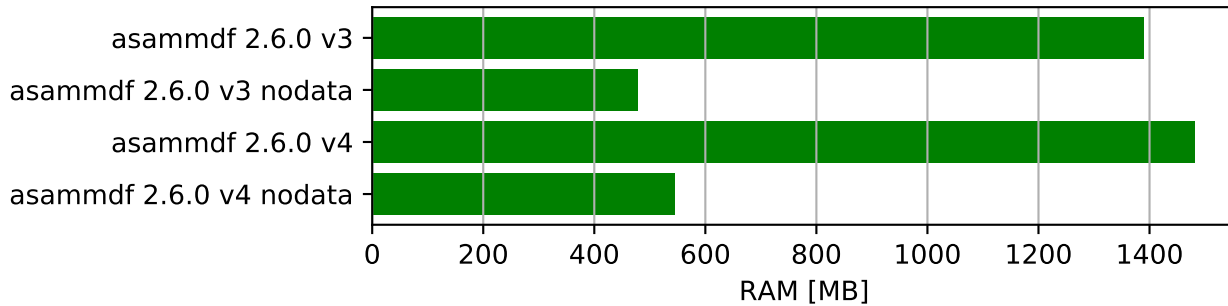
Merge test file - ram usage
