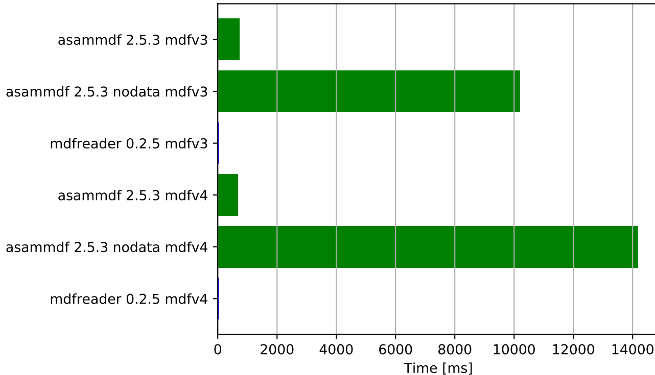
Get all channels (36424 calls) - time
