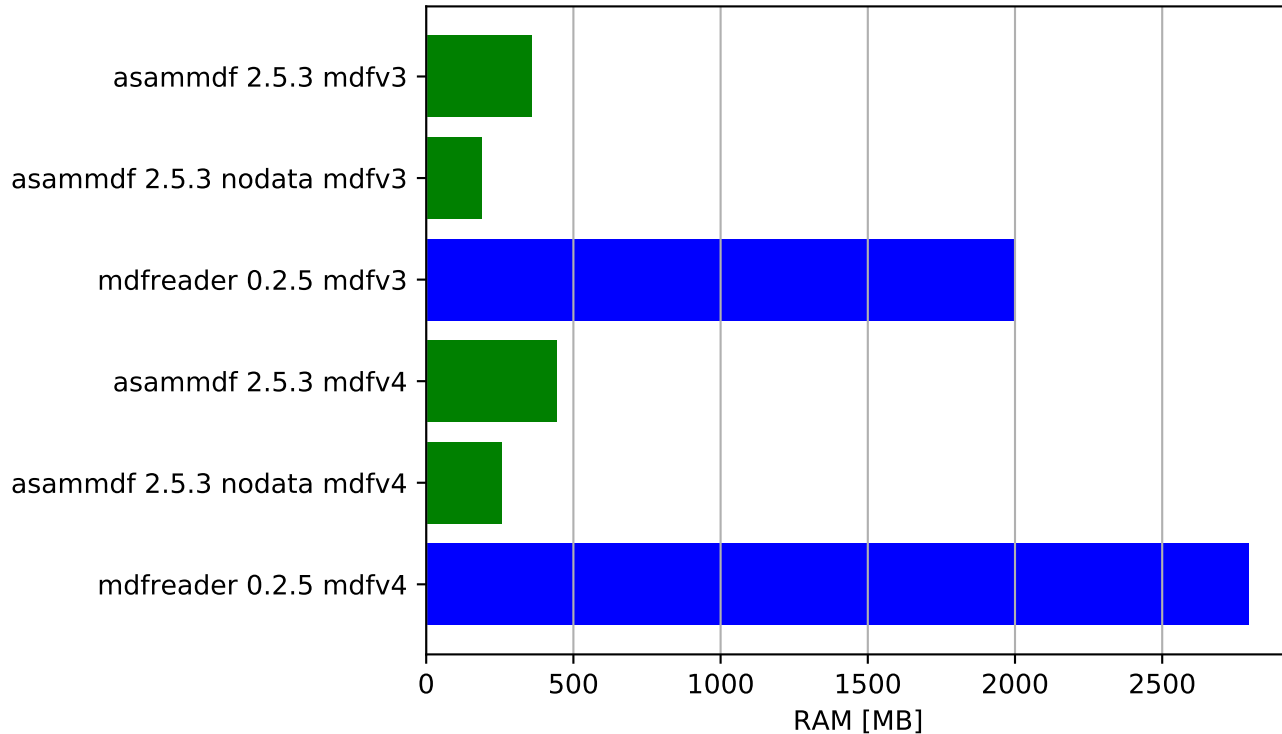
Save test file - ram usage
