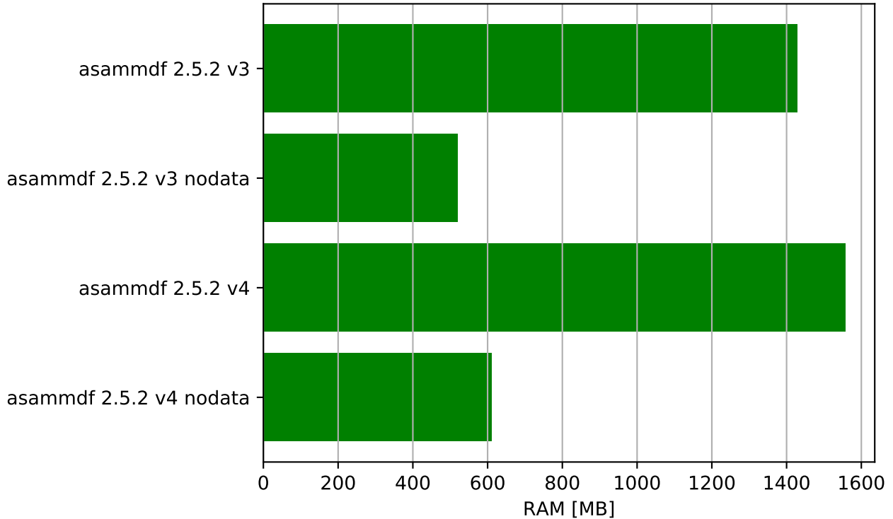
Merge test file - ram usage
