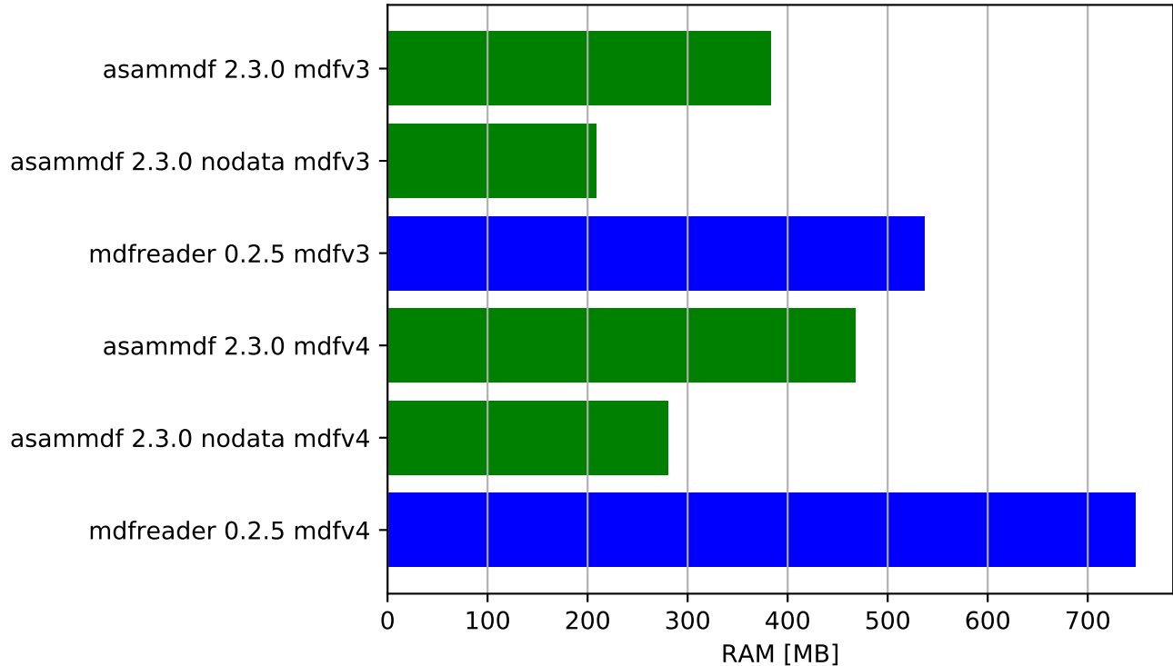
Get all channels (36424 calls) - ram usage
