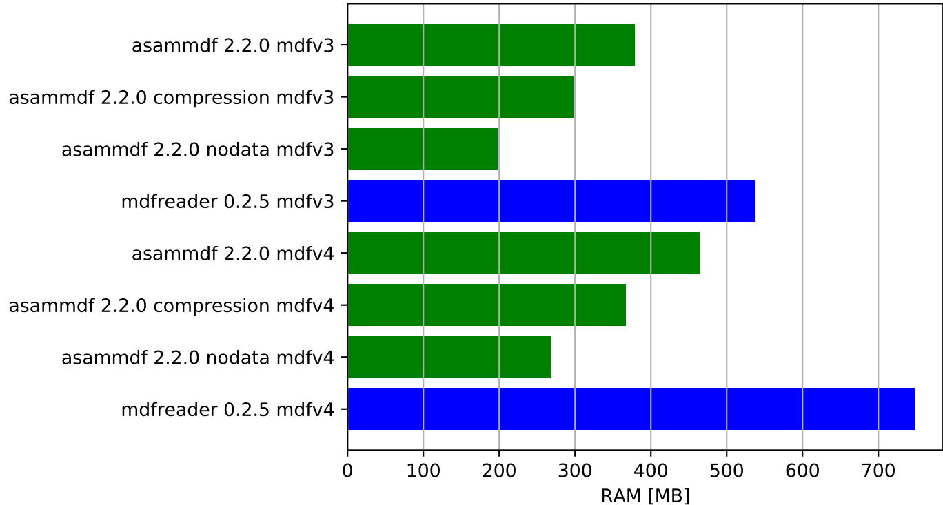
Open test file - ram usage
