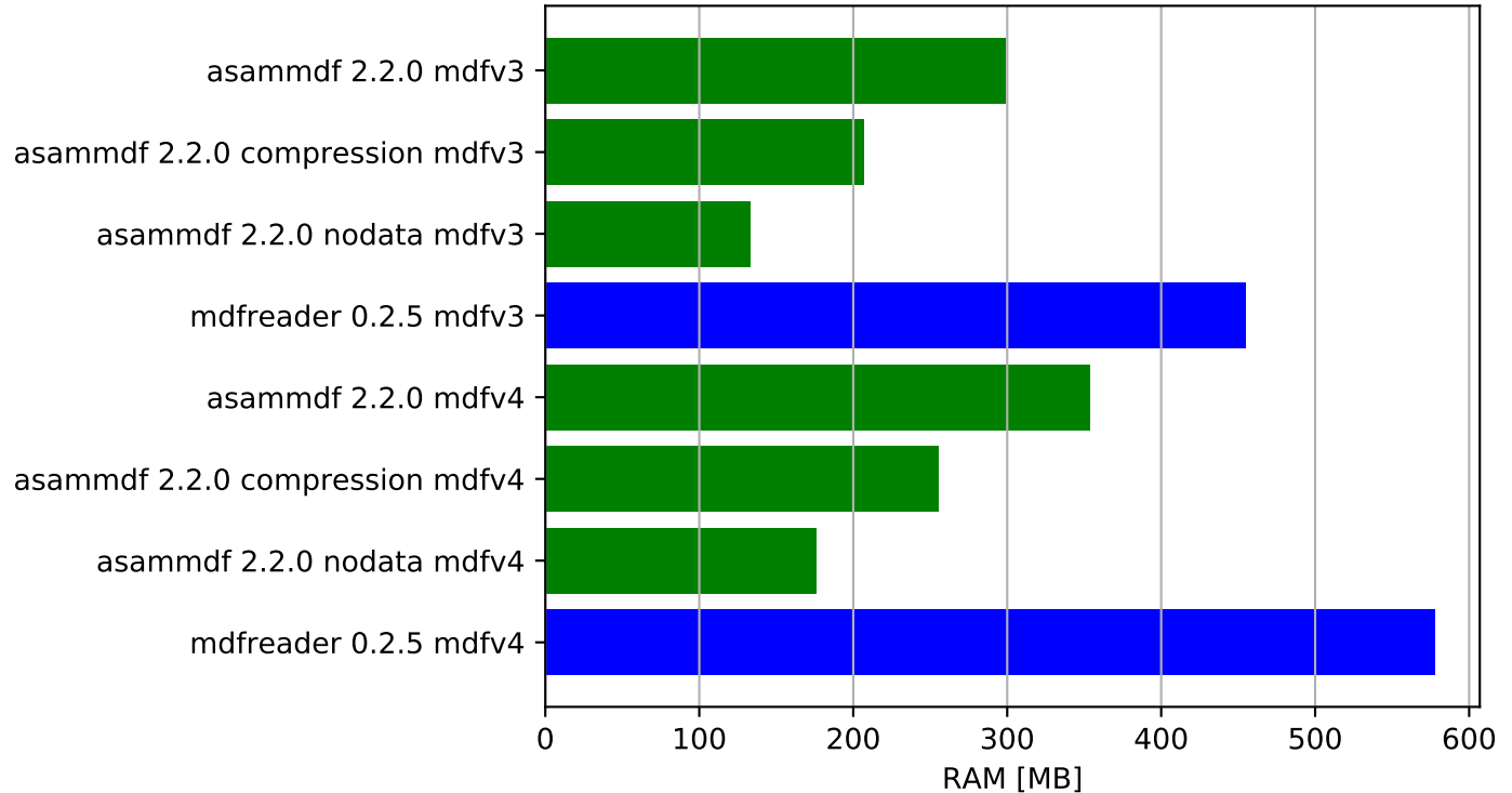
Get all channels (36424 calls) - ram usage
