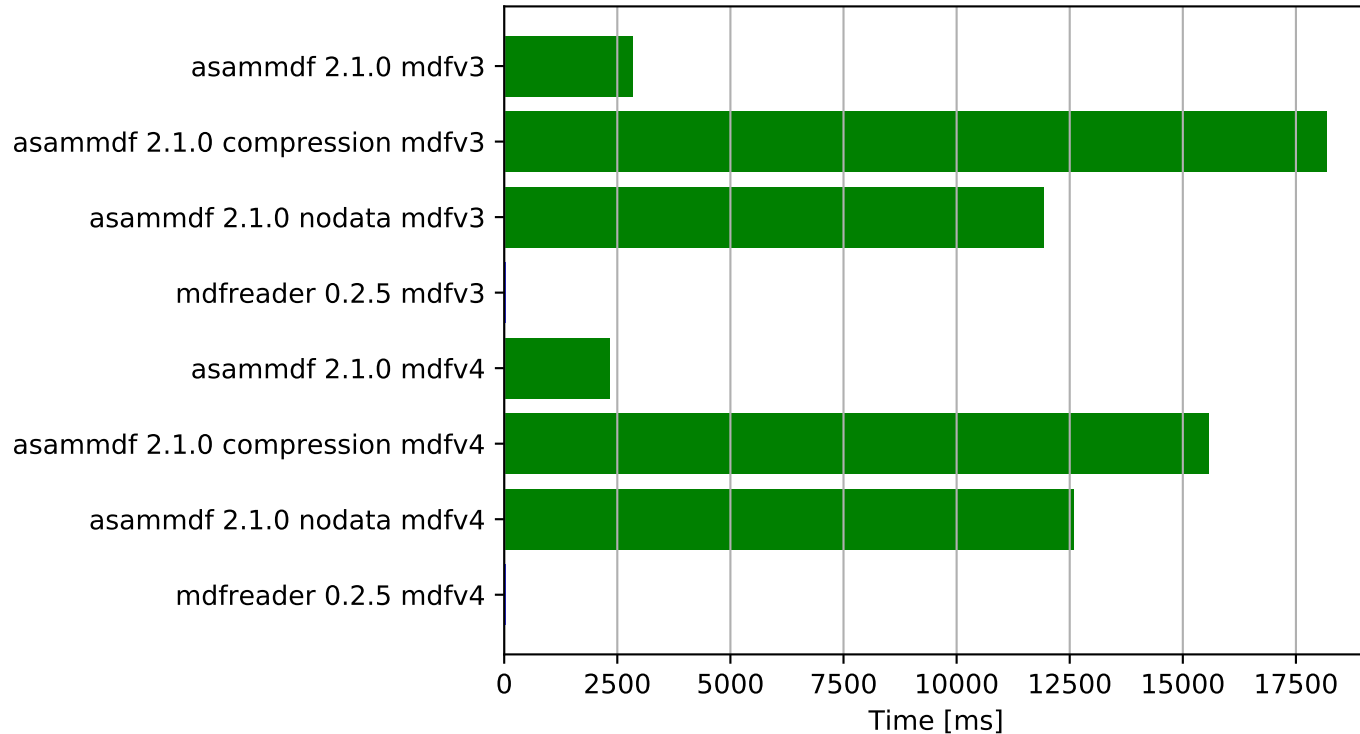
Get all channels (36424 calls) - time
