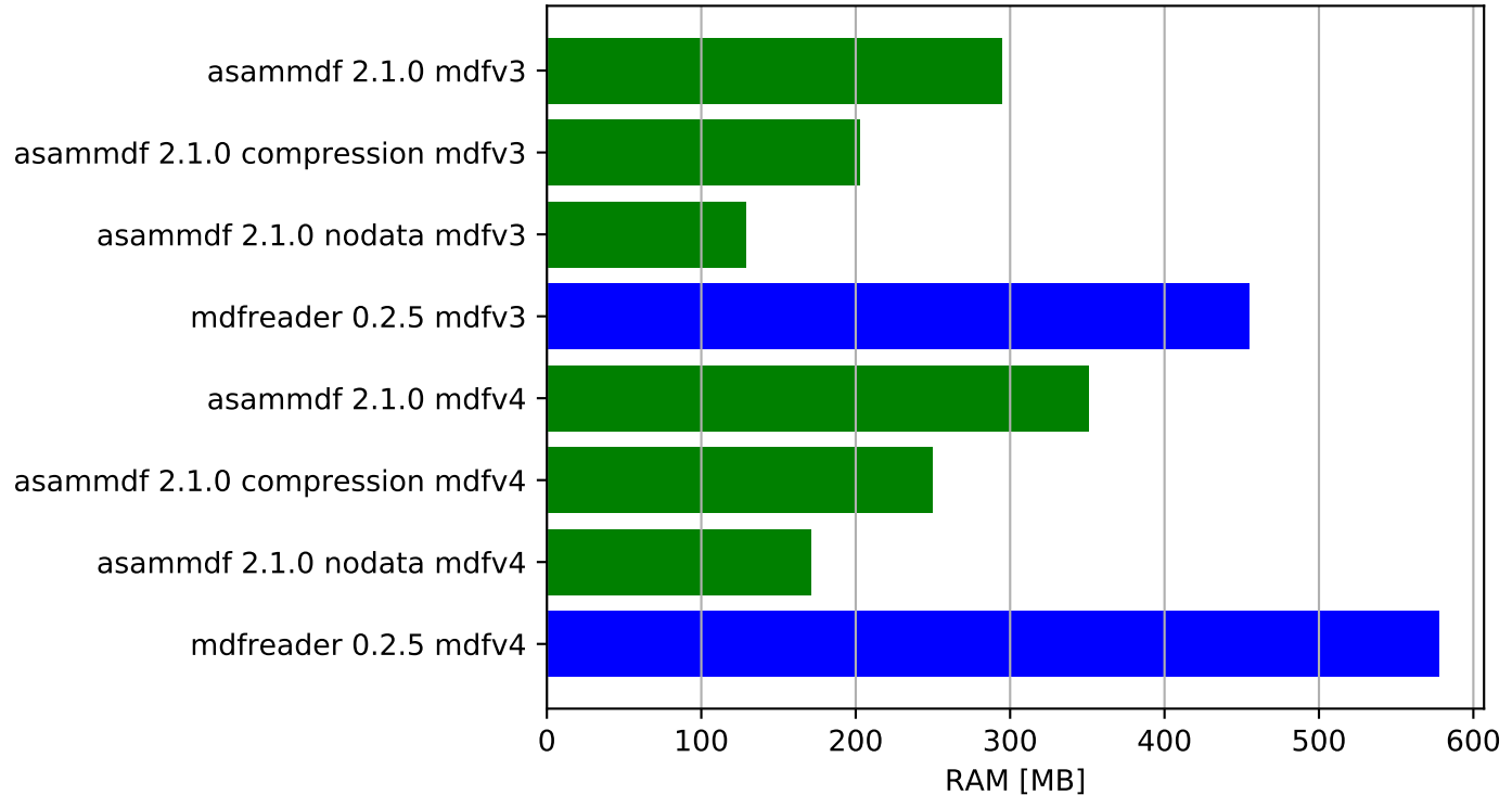
Get all channels (36424 calls) - RAM usage
